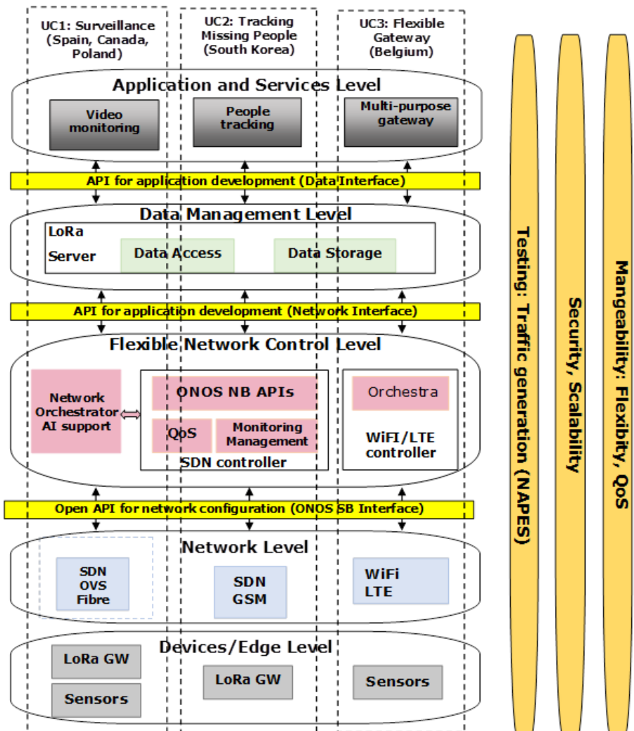
FlexNet architecture
