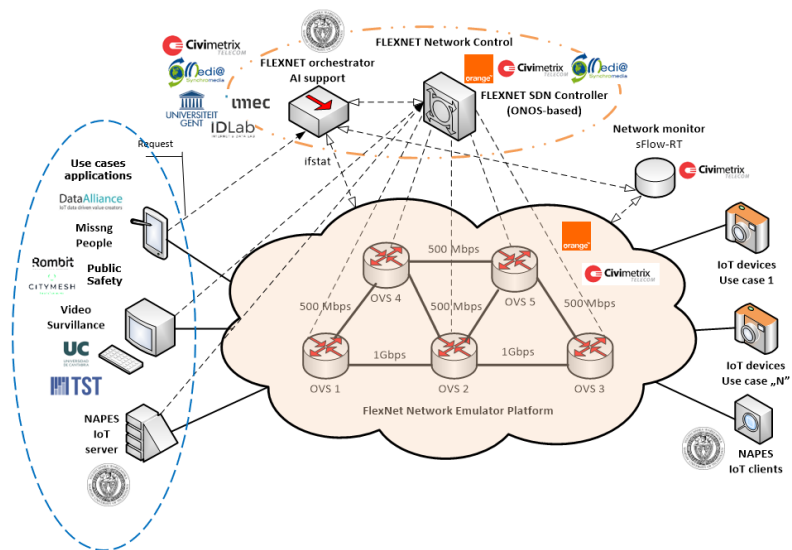
FlexNet implementation
